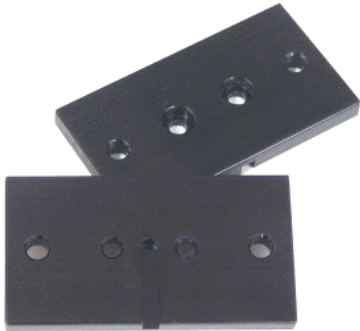
Base Mounting plates. Top plate showing the countersunk holes in the centre of the plate that are used to attach the base. Lower plate showing the cable groove.
