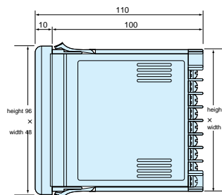
SR74A External dimensions
