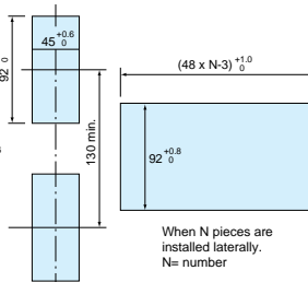
SR74A Panel cutout
