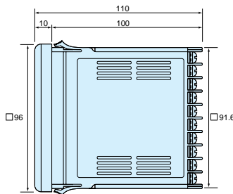
SR73A External dimensions
