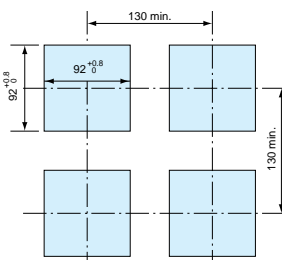
SR73A Panel cutout
